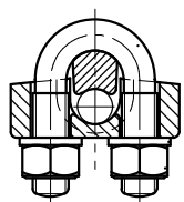
SECTION Y-Y
